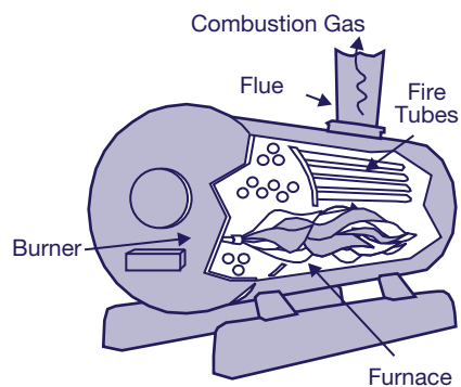
Figure 6: Boiler Components
