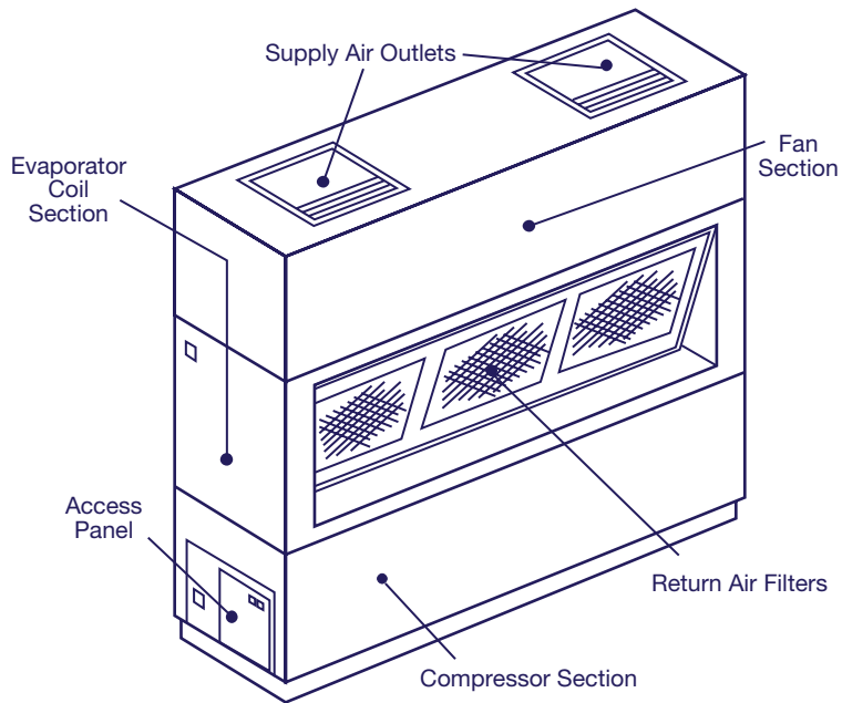
Figure 9: Vertical Packaged Units
