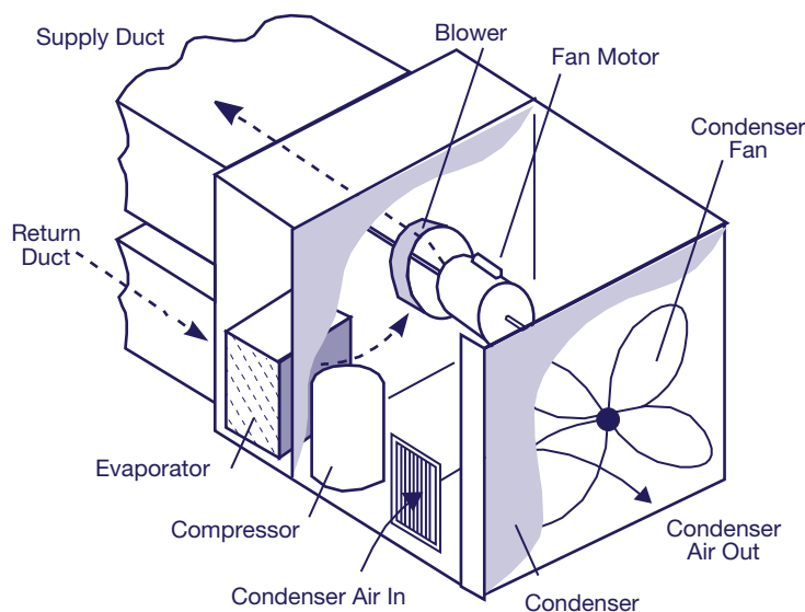
Figure 8: Self-Contained Packaged AC Unit
