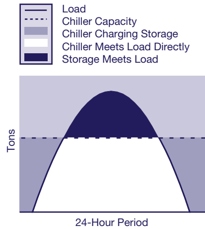
Figure 12: Partial-Storage Strategy
